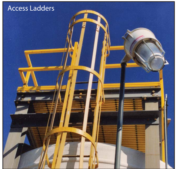
Fiberglass Platforms | Ciba Geigy Plant
