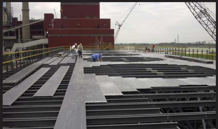
SAFDECK is lightweight and easy to install, especially in rooftop applications like this cooling tower fan deck. The quick screw-down construction of the SAFDECK system ensures rapid installation and reduced field labor costs.
